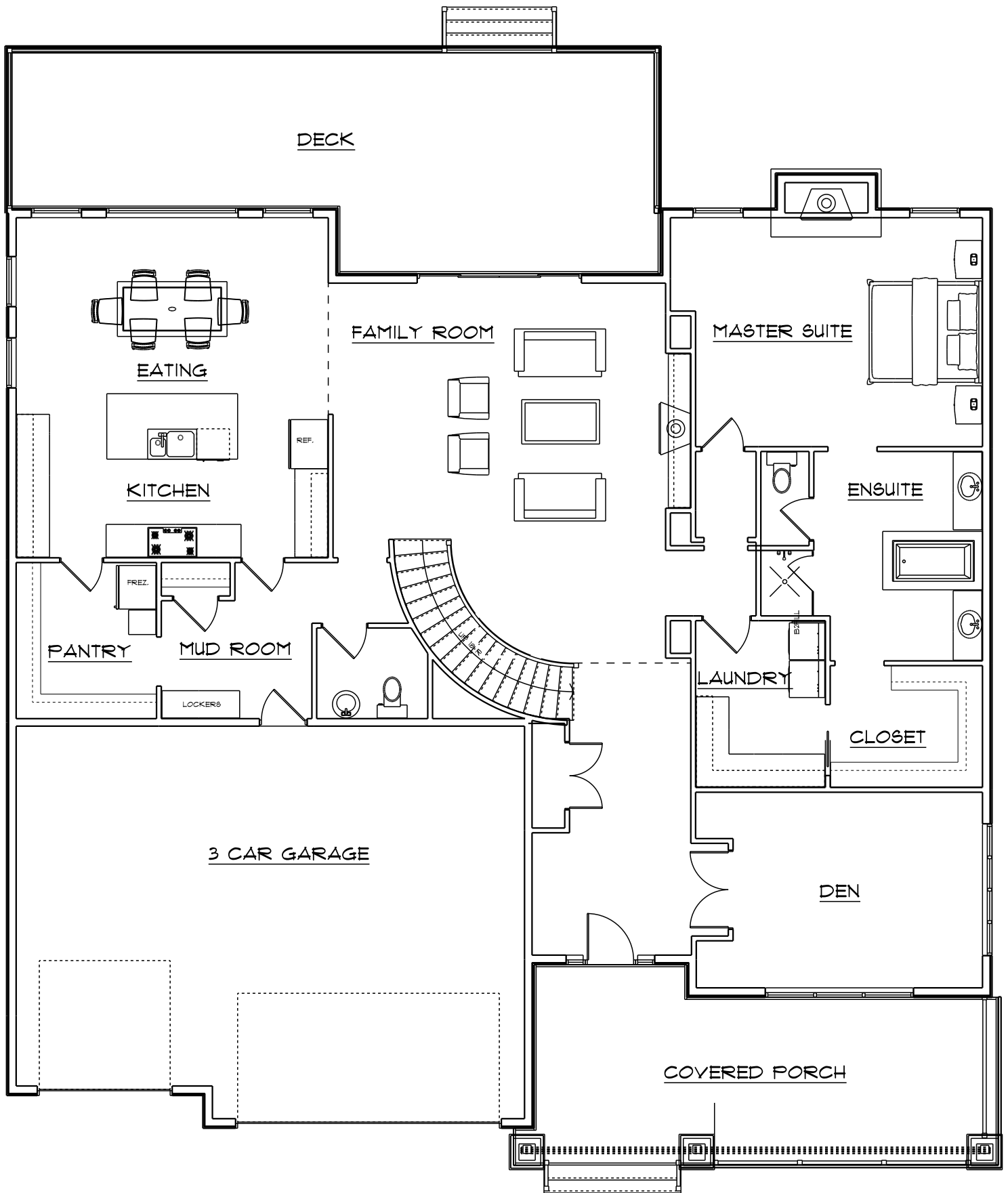
MAIN FLOOR 2245 SQ.FT.
