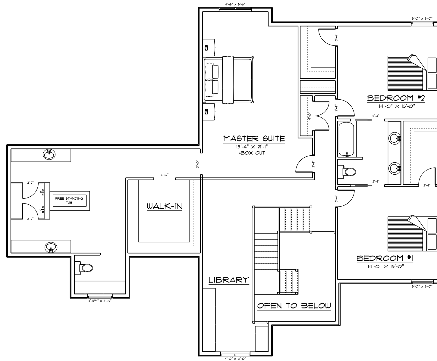
2ND FLOOR LAYOUT 1860 SQ.FT.
