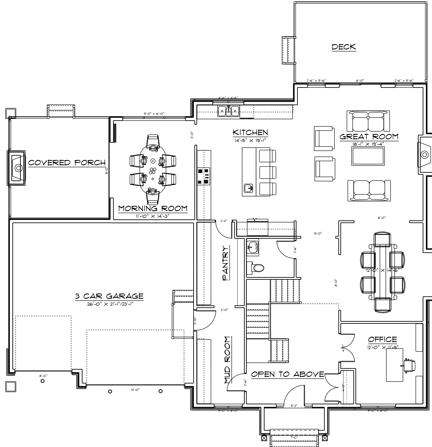
MAIN FLOOR LAYOUT 1756 SQ.FT.
