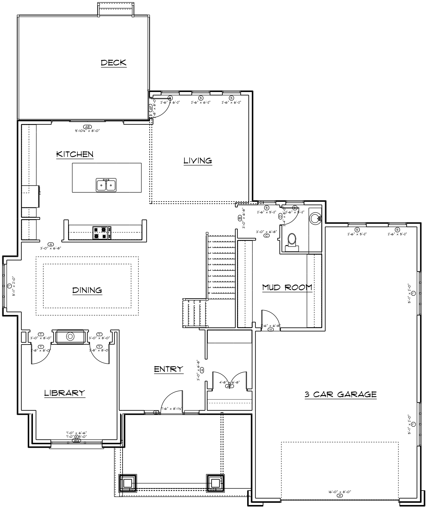
MAIN FLOOR PLAN 1360 sq.ft
