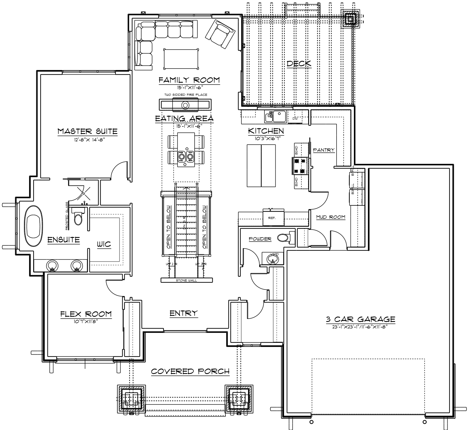
MAIN FLOOR LAYOUT 1721 SF
