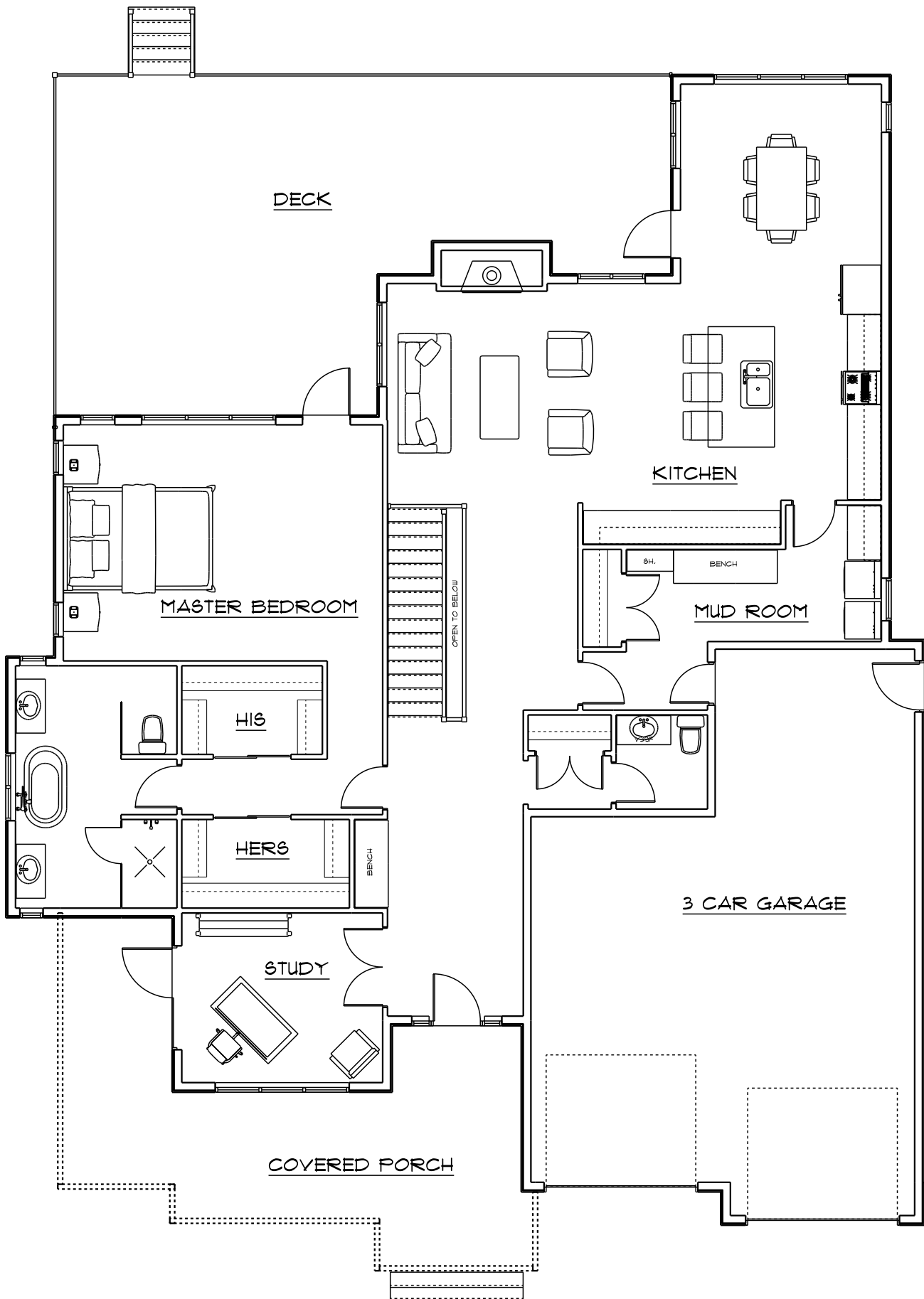
MAIN FLOOR PLAN 1947 SF
